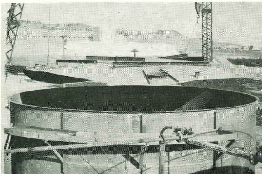
These pictures taken during the installation of No. 8 acid storage tank show the top cover plate being lifted into position (top), and ready to be dropped in place (bottom).
